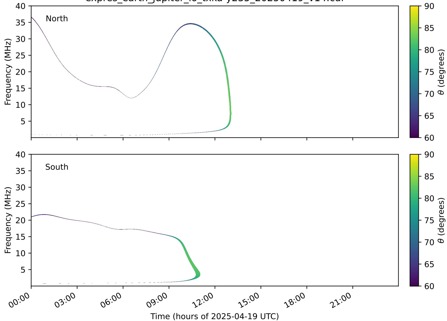
expres_earth_jupiter_io_txka-y235_20250419_v14.cdf
