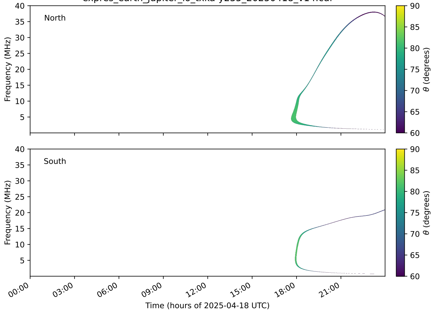
expres_earth_jupiter_io_txka-y235_20250418_v14.cdf
