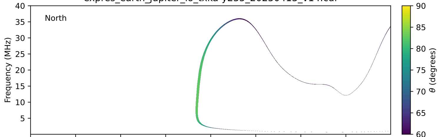
expres_earth_jupiter_io_txka-y235_20250413_v14.cdf
