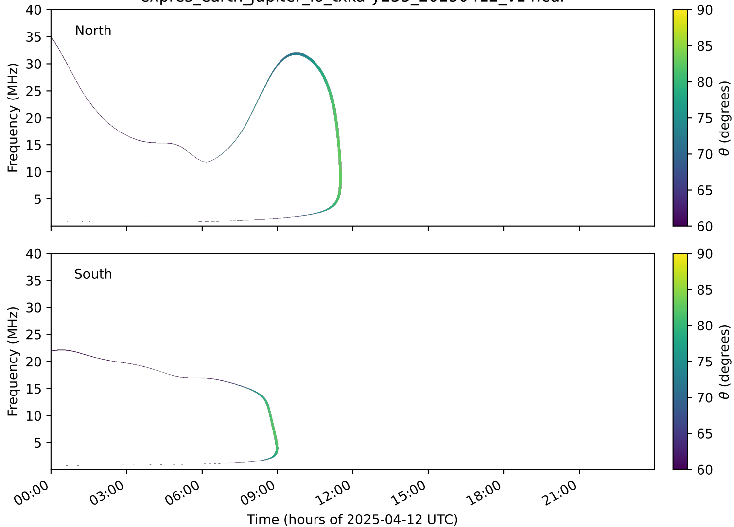
expres_earth_jupiter_io_txka-y235_20250412_v14.cdf
