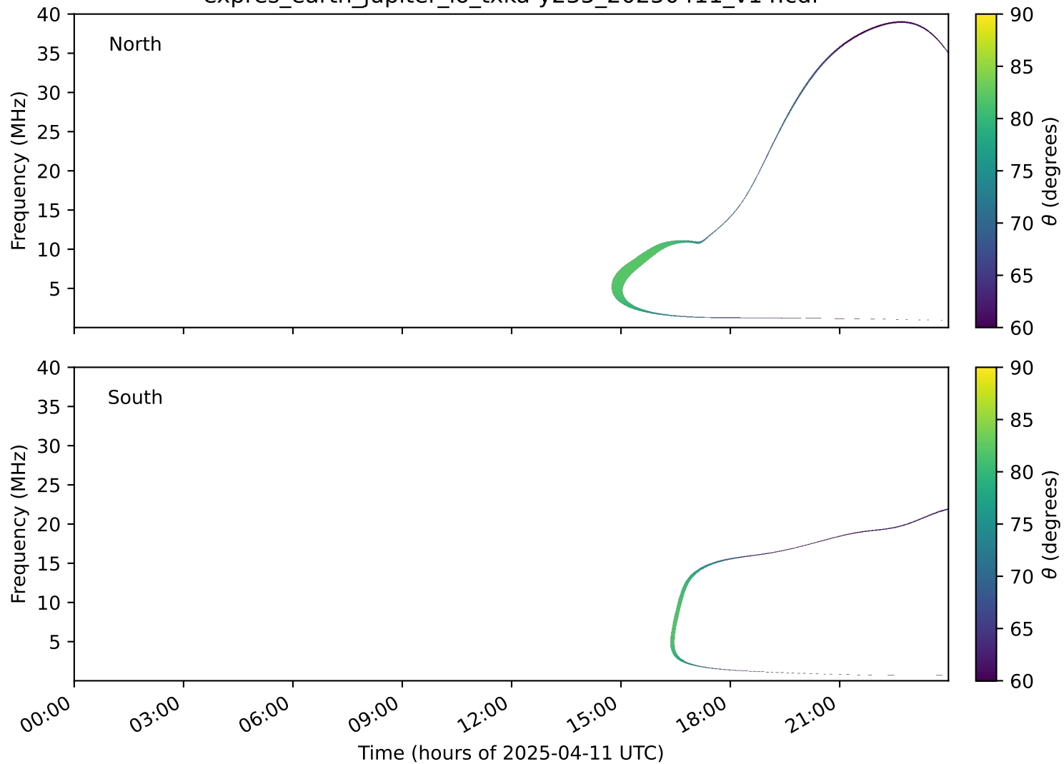
expres_earth_jupiter_io_txka-y235_20250411_v14.cdf
