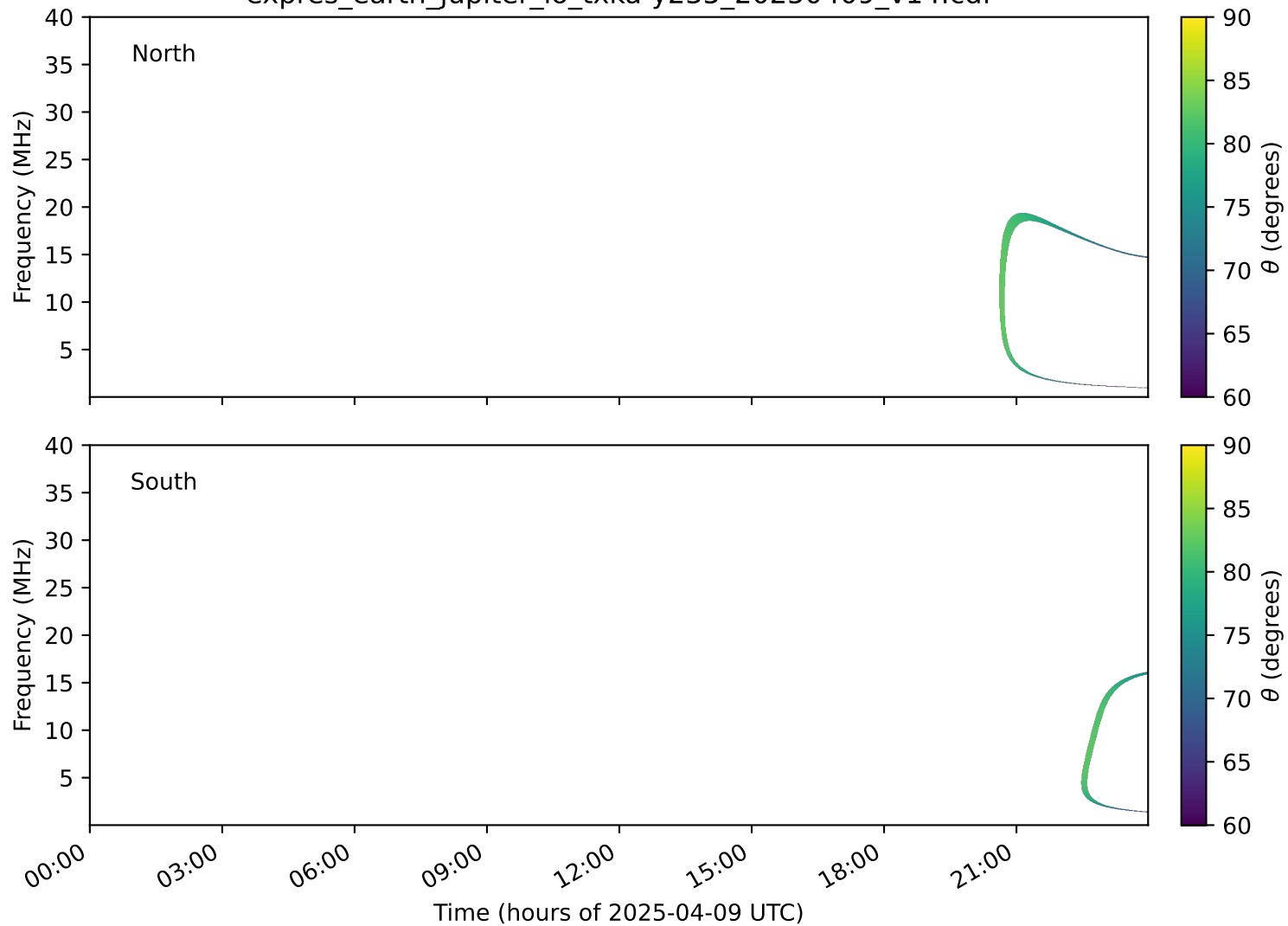
expres_earth_jupiter_io_txka-y235_20250409_v14.cdf
