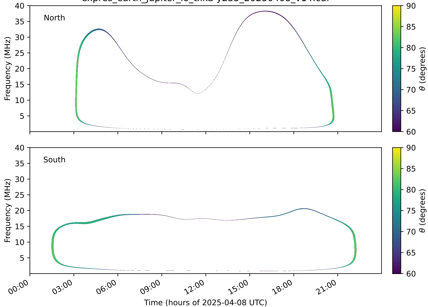
expres_earth_jupiter_io_txka-y235_20250408_v14.cdf
