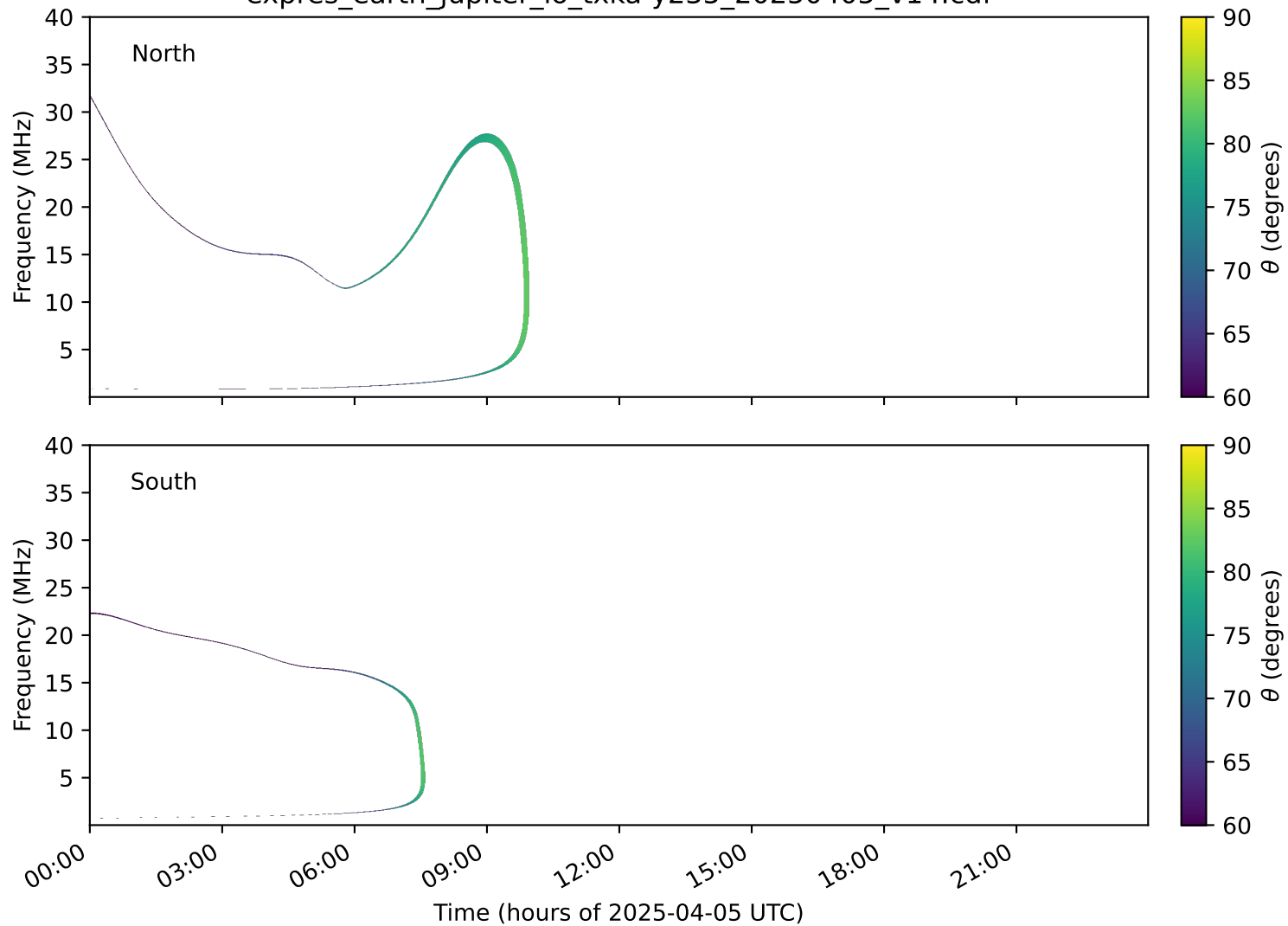
expres_earth_jupiter_io_txka-y235_20250405_v14.cdf
