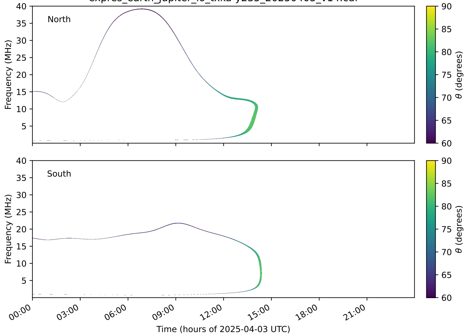
expres_earth_jupiter_io_txka-y235_20250403_v14.cdf
