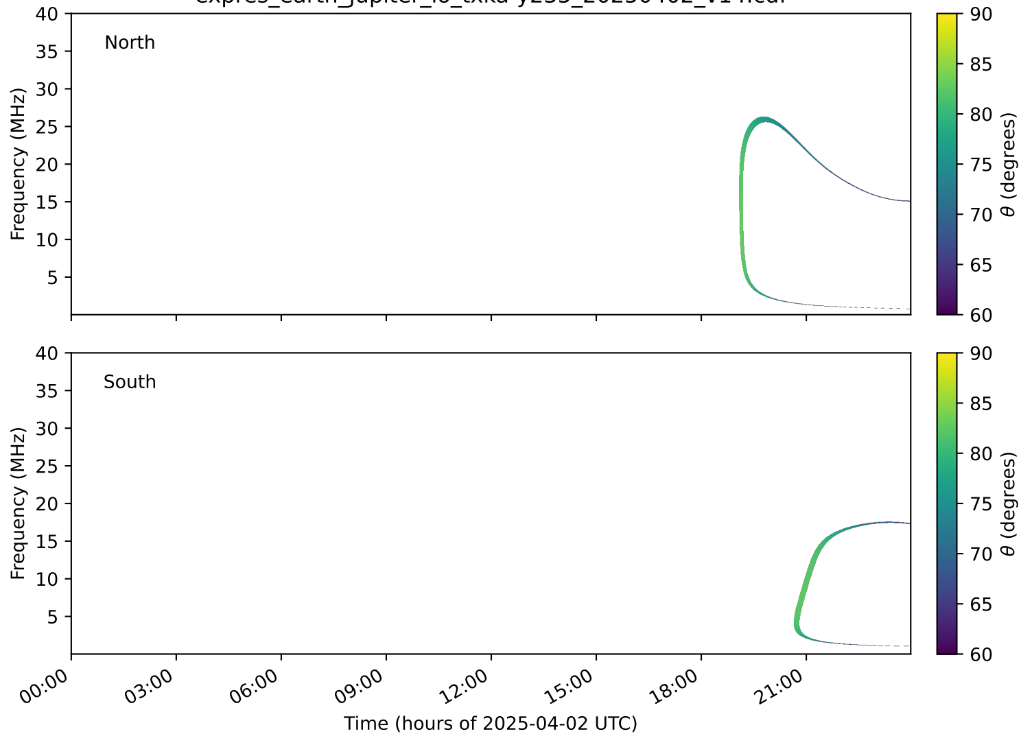
expres_earth_jupiter_io_txka-y235_20250402_v14.cdf
