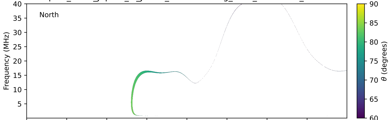
expres_earth_jupiter_io_jrm33_lossc-wid1deg_3kev_20250429_v11.cdf
