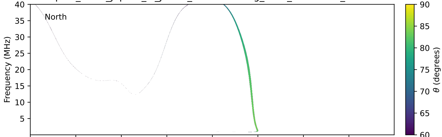
expres_earth_jupiter_io_jrm33_lossc-wid1deg_3kev_20250426_v11.cdf
