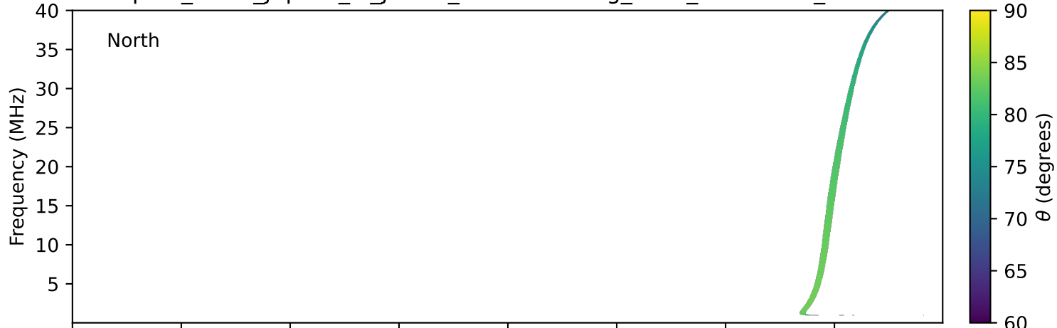
expres_earth_jupiter_io_jrm33_lossc-wid1deg_3kev_20250425_v11.cdf
