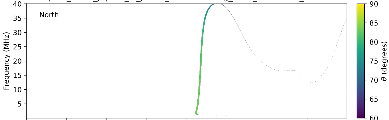
expres_earth_jupiter_io_jrm33_lossc-wid1deg_3kev_20250420_v11.cdf
