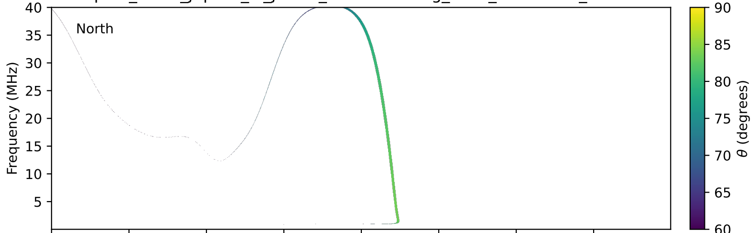
expres_earth_jupiter_io_jrm33_lossc-wid1deg_3kev_20250419_v11.cdf
