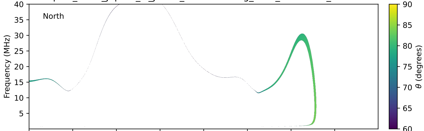
expres_earth_jupiter_io_jrm33_lossc-wid1deg_3kev_20250417_v11.cdf
