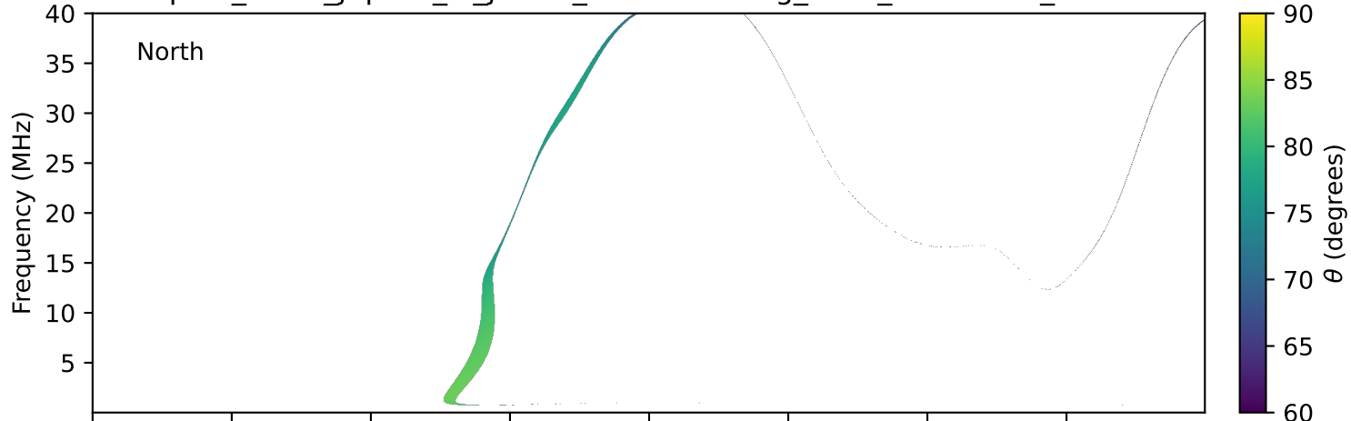
expres_earth_jupiter_io_jrm33_lossc-wid1deg_3kev_20250406_v11.cdf
