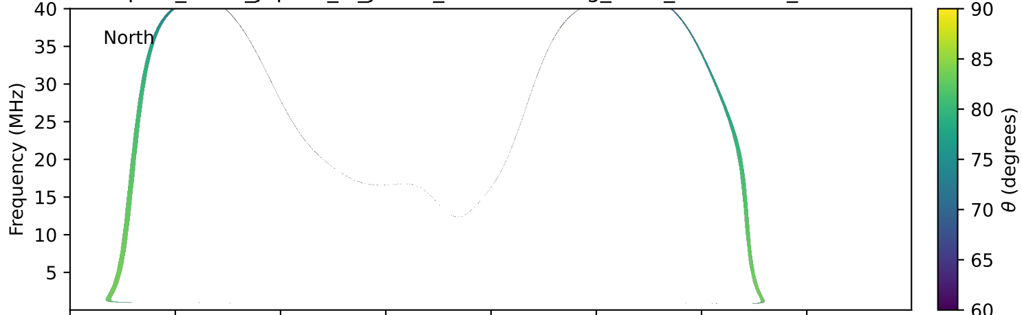
expres_earth_jupiter_io_jrm33_lossc-wid1deg_3kev_20250401_v11.cdf
