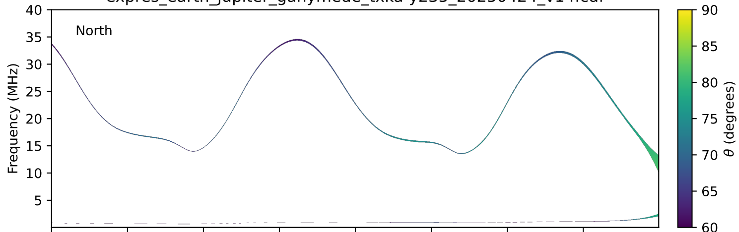
expres_earth_jupiter_ganymede_txka-y235_20250424_v14.cdf
