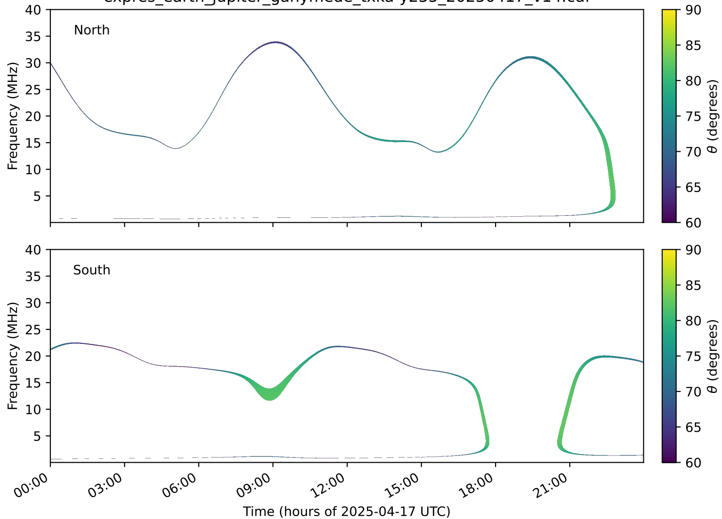
expres_earth_jupiter_ganymede_txka-y235_20250417_v14.cdf
