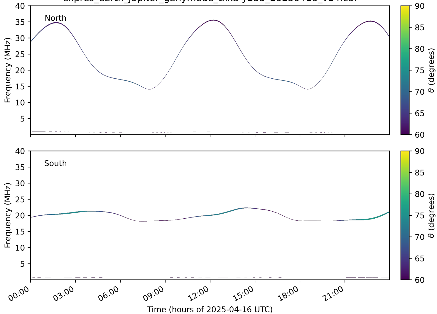
expres_earth_jupiter_ganymede_txka-y235_20250416_v14.cdf
