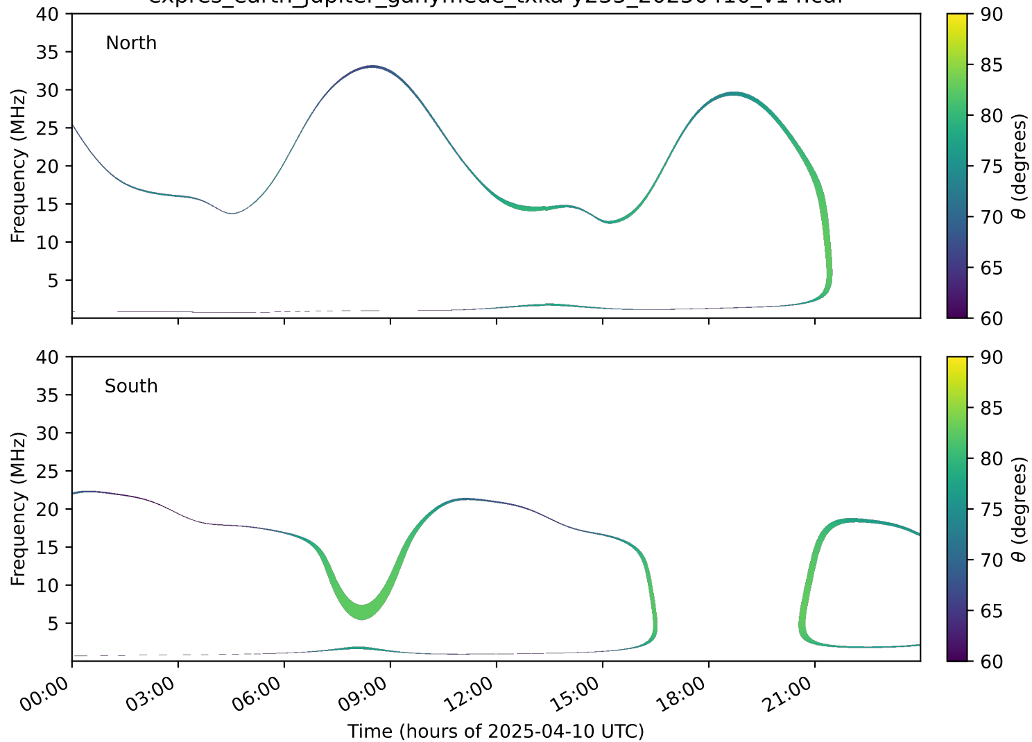
expres_earth_jupiter_ganymede_txka-y235_20250410_v14.cdf
