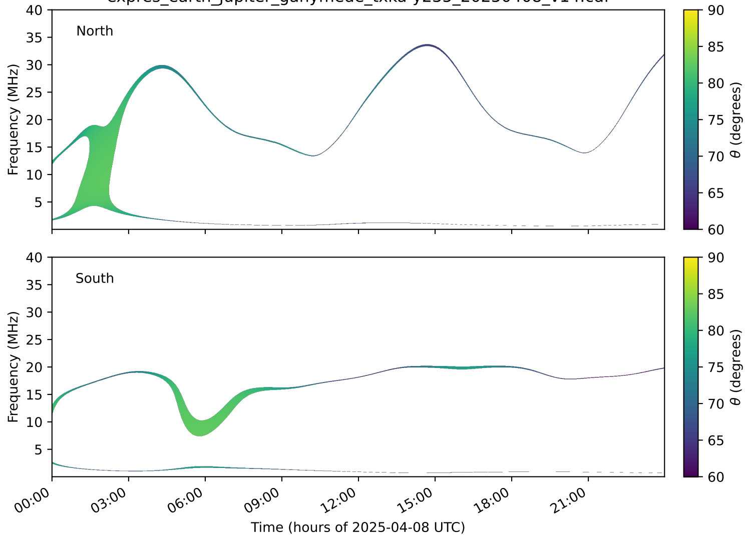
expres_earth_jupiter_ganymede_txka-y235_20250408_v14.cdf
