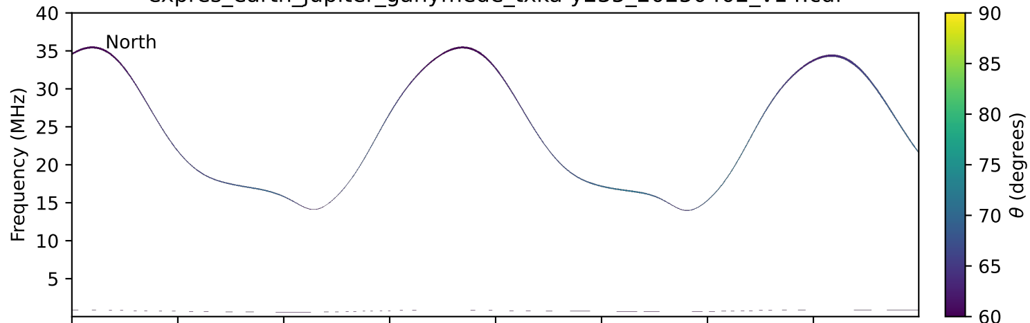
expres_earth_jupiter_ganymede_txka-y235_20250402_v14.cdf
