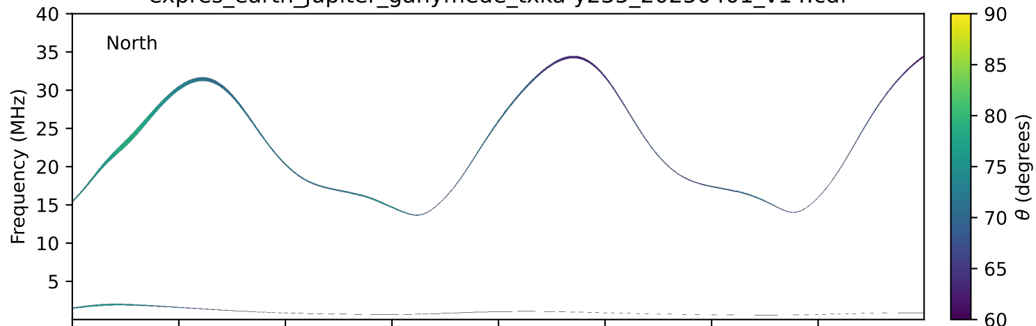
expres_earth_jupiter_ganymede_txka-y235_20250401_v14.cdf
