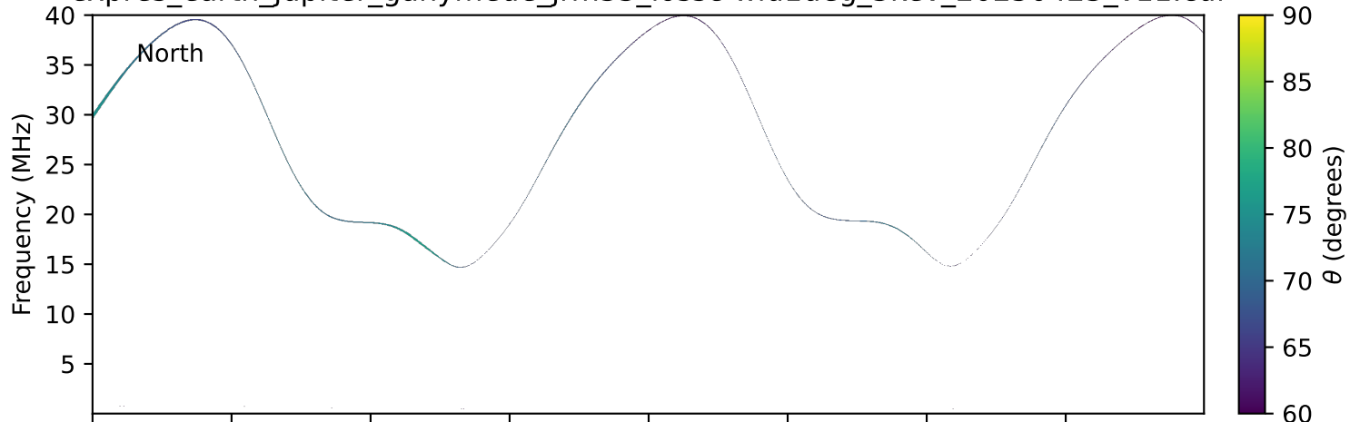
expres_earth_jupiter_ganymede_jrm33_lossc-wid1deg_3kev_20250423_v11.cdf
