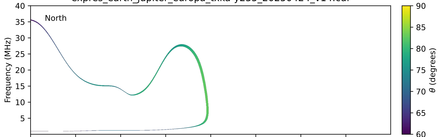
expres_earth_jupiter_europa_txka-y235_20250424_v14.cdf
