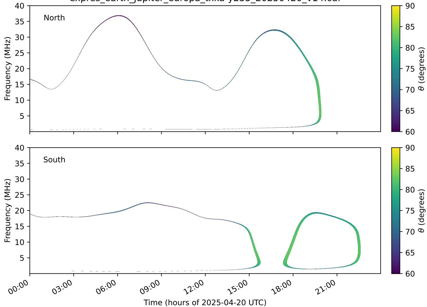
expres_earth_jupiter_europa_txka-y235_20250420_v14.cdf
