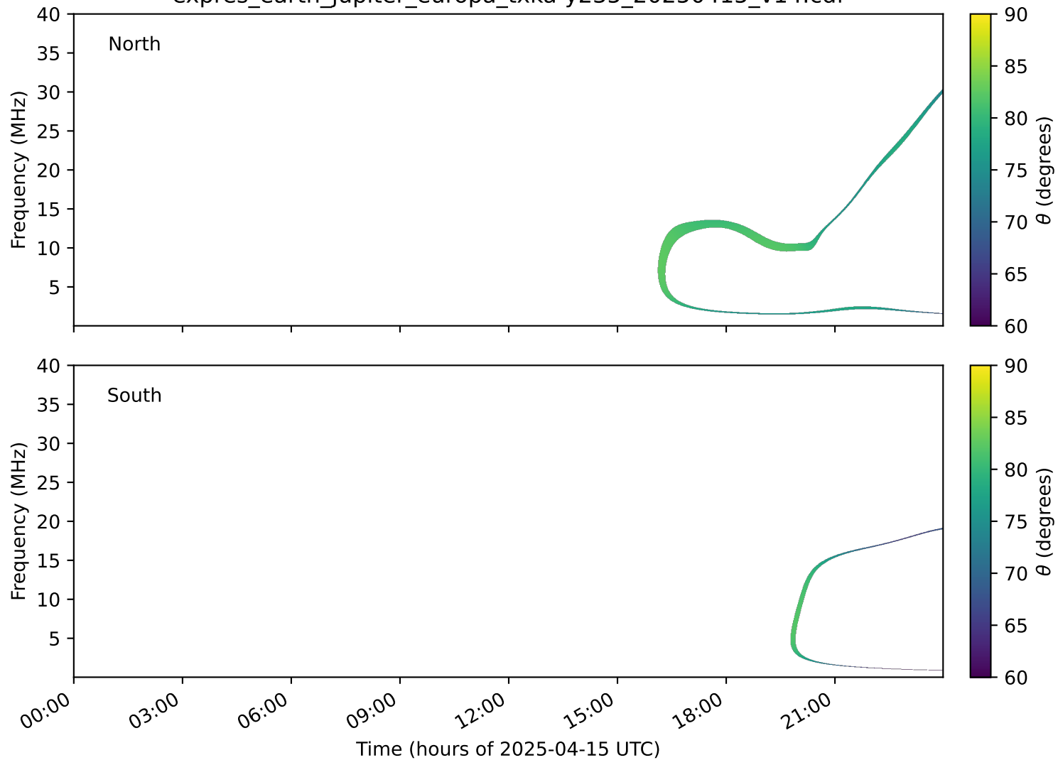
expres_earth_jupiter_europa_txka-y235_20250415_v14.cdf
