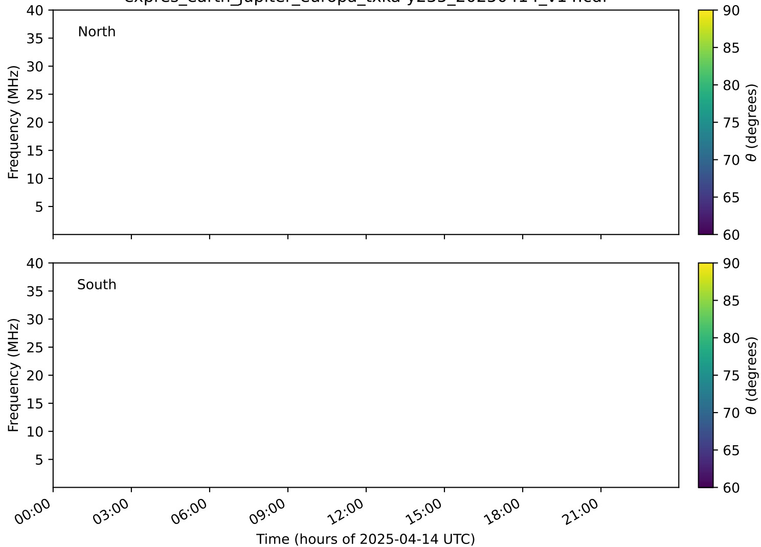
expres_earth_jupiter_europa_txka-y235_20250414_v14.cdf
