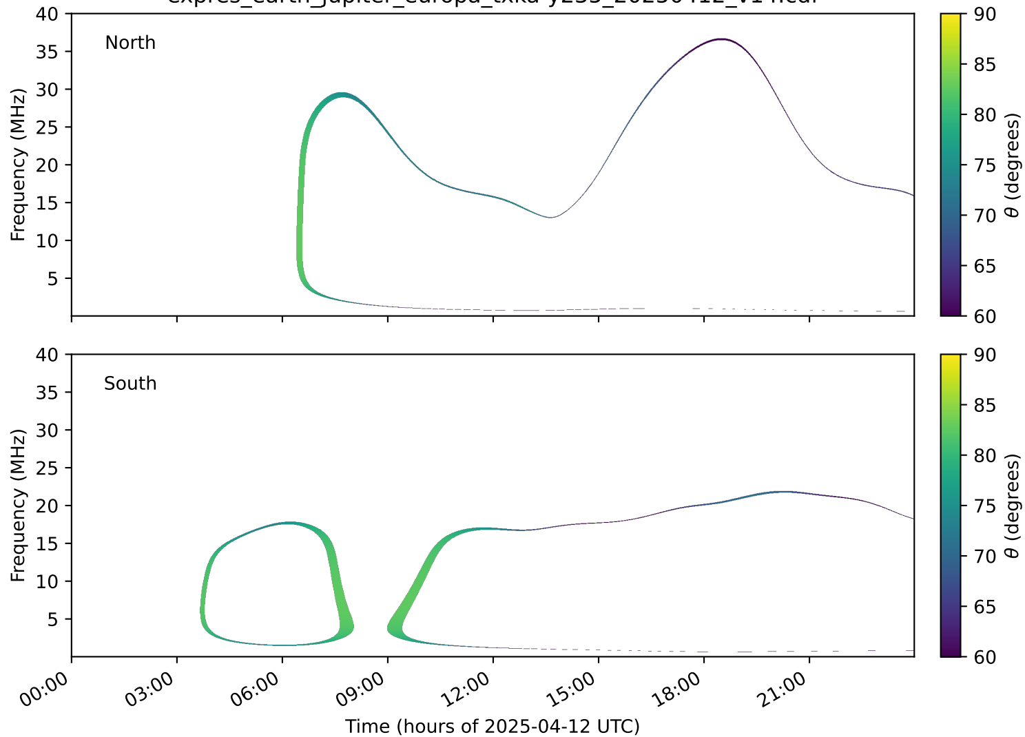
expres_earth_jupiter_europa_txka-y235_20250412_v14.cdf
