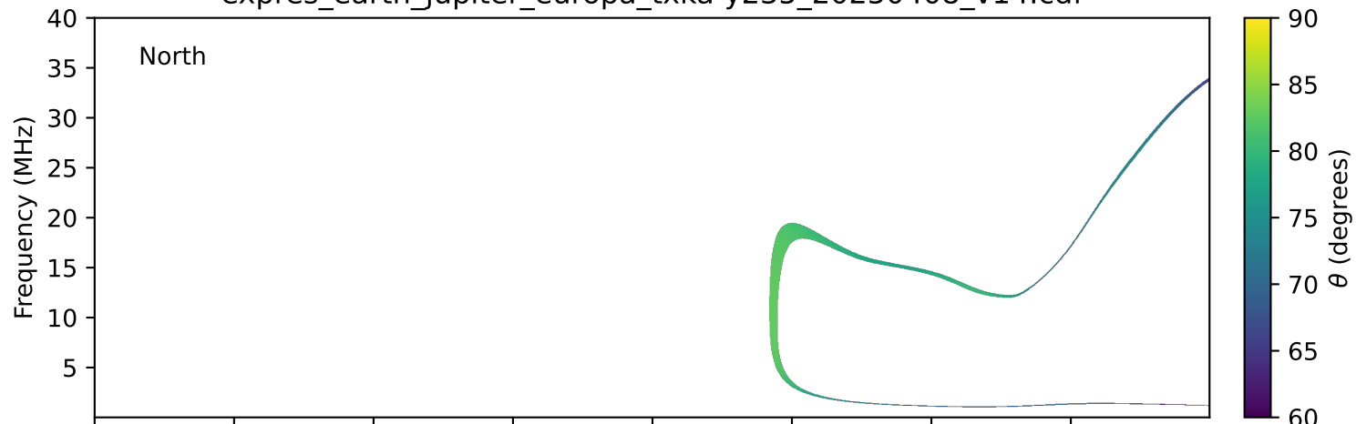
expres_earth_jupiter_europa_txka-y235_20250408_v14.cdf
