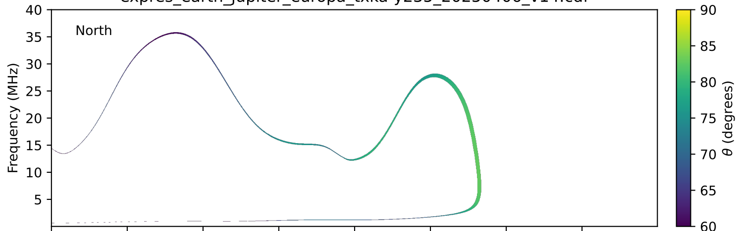
expres_earth_jupiter_europa_txka-y235_20250406_v14.cdf
