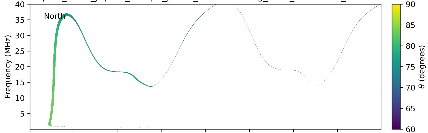
expres_earth_jupiter_europa_jrm33_lossc-wid1deg_3kev_20250430_v11.cdf
