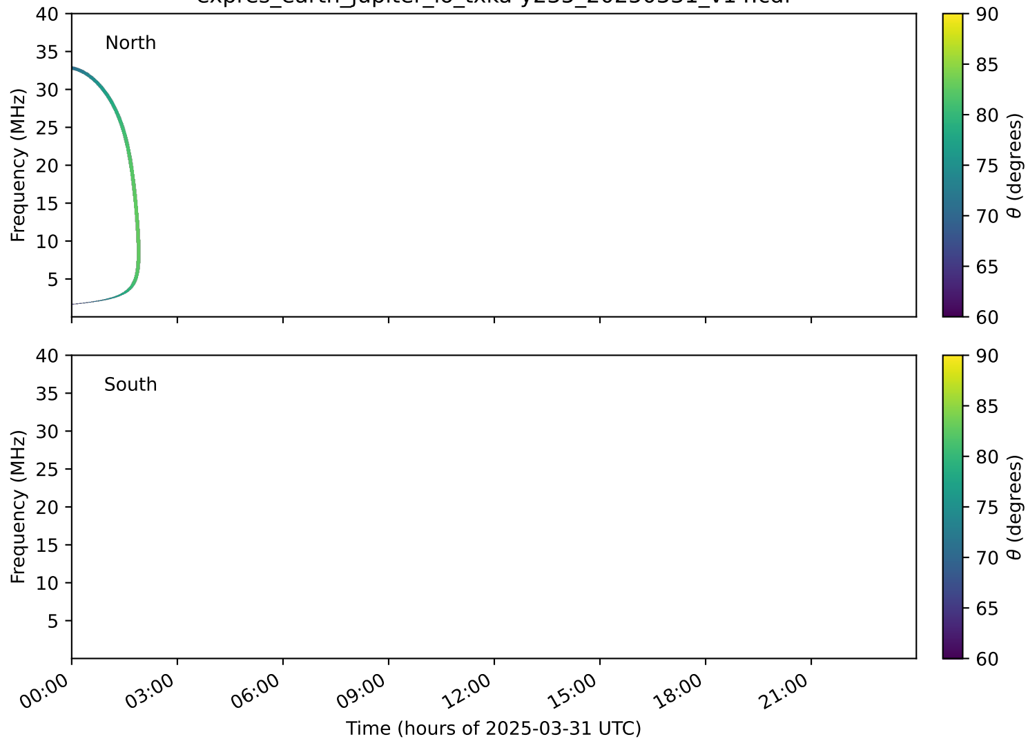
expres_earth_jupiter_io_txka-y235_20250331_v14.cdf
