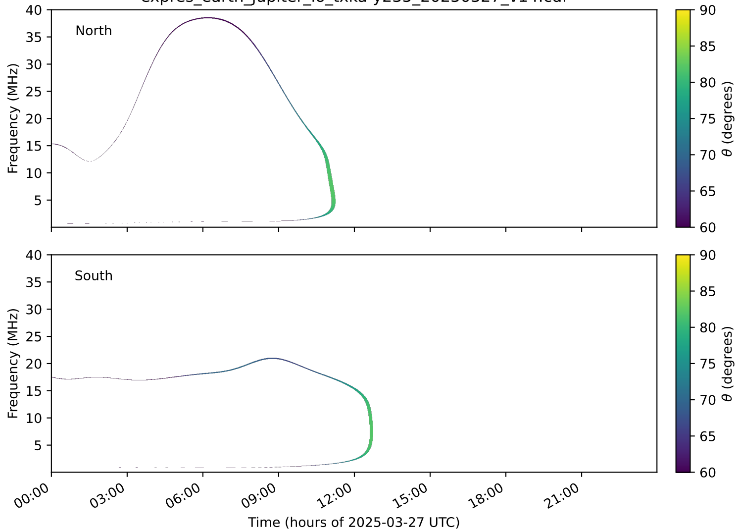
expres_earth_jupiter_io_txka-y235_20250327_v14.cdf
