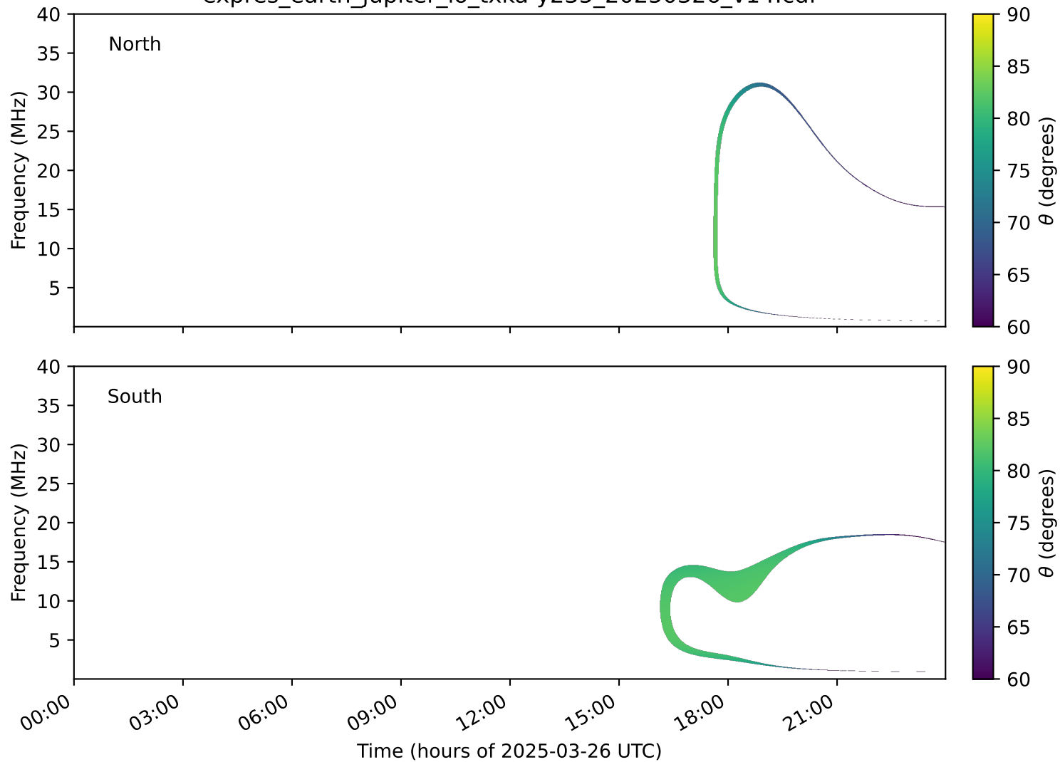
expres_earth_jupiter_io_txka-y235_20250326_v14.cdf
