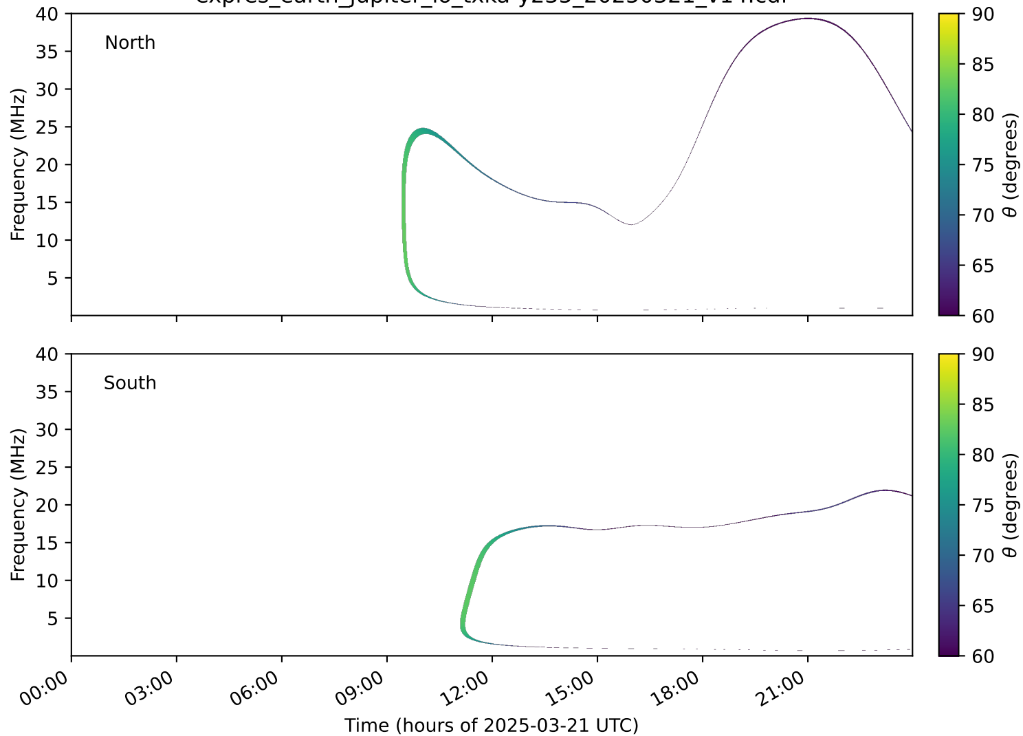
expres_earth_jupiter_io_txka-y235_20250321_v14.cdf
