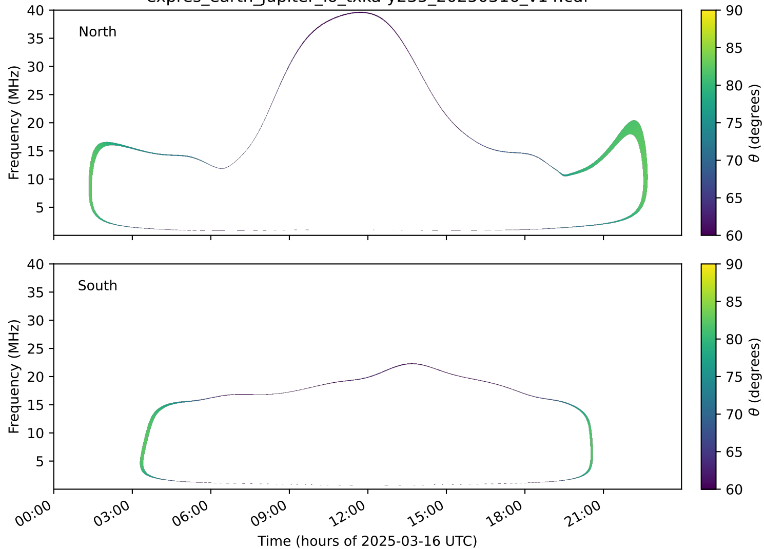
expres_earth_jupiter_io_txka-y235_20250316_v14.cdf
