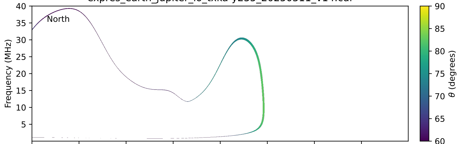
expres_earth_jupiter_io_txka-y235_20250311_v14.cdf
