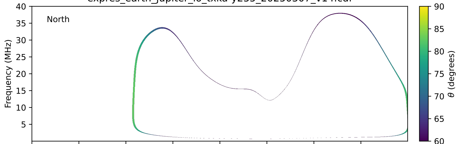
expres_earth_jupiter_io_txka-y235_20250307_v14.cdf
