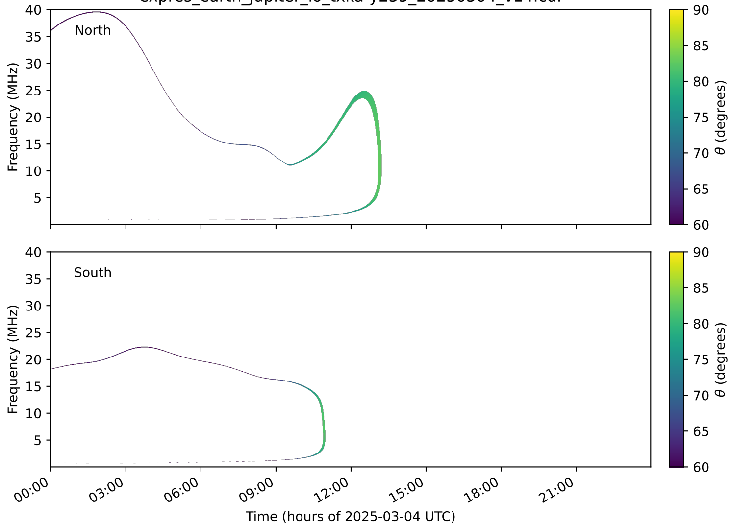
expres_earth_jupiter_io_txka-y235_20250304_v14.cdf
