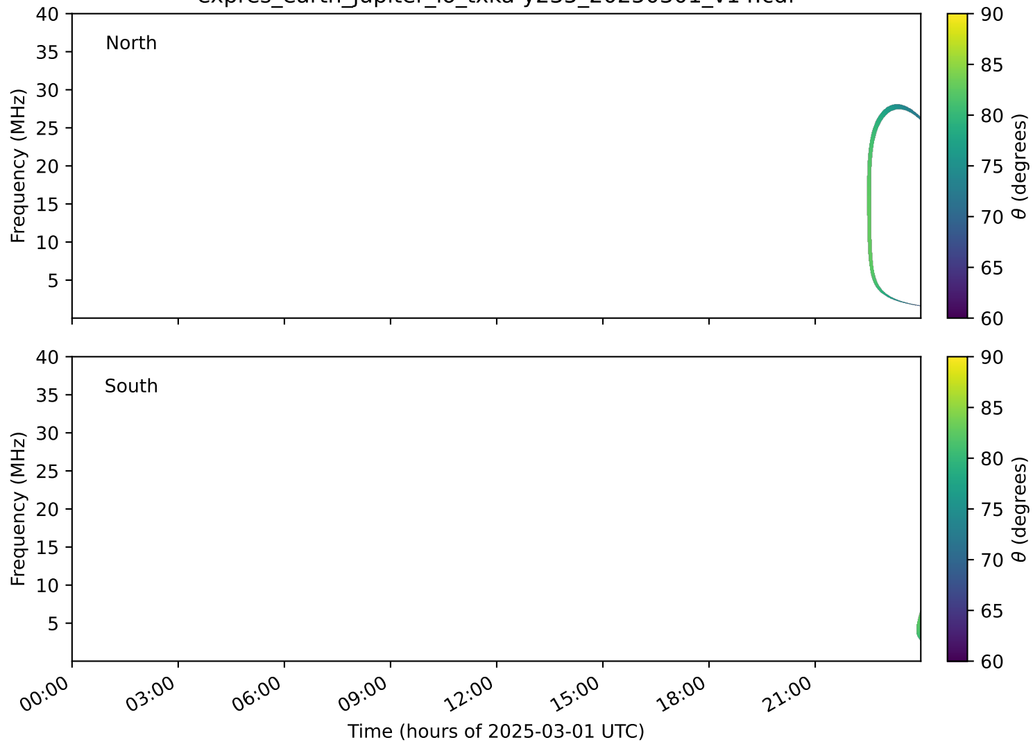
expres_earth_jupiter_io_txka-y235_20250301_v14.cdf
