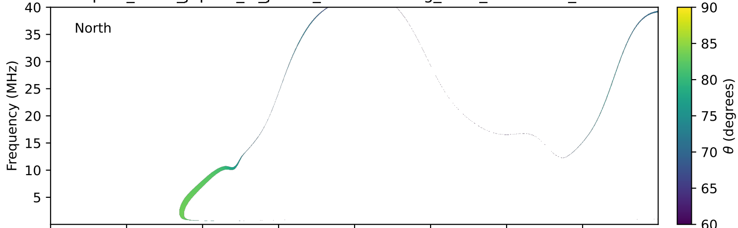
expres_earth_jupiter_io_jrm33_lossc-wid1deg_3kev_20250330_v11.cdf
