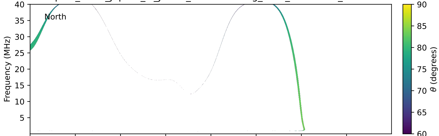
expres_earth_jupiter_io_jrm33_lossc-wid1deg_3kev_20250325_v11.cdf
