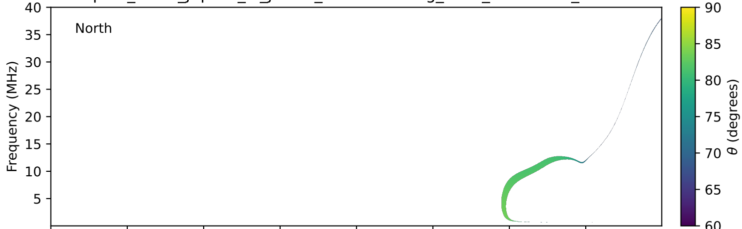
expres_earth_jupiter_io_jrm33_lossc-wid1deg_3kev_20250310_v11.cdf
