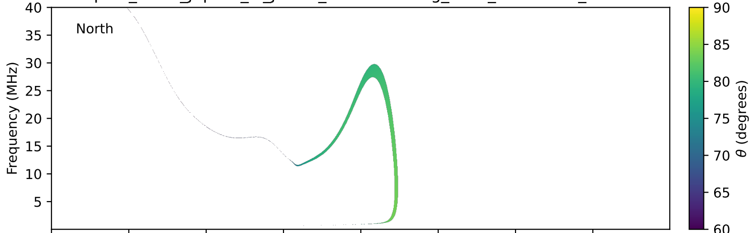
expres_earth_jupiter_io_jrm33_lossc-wid1deg_3kev_20250304_v11.cdf
