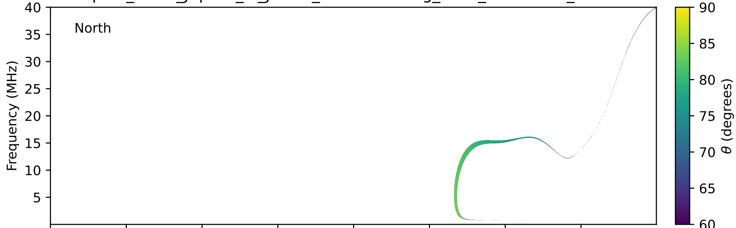
expres_earth_jupiter_io_jrm33_lossc-wid1deg_3kev_20250303_v11.cdf
