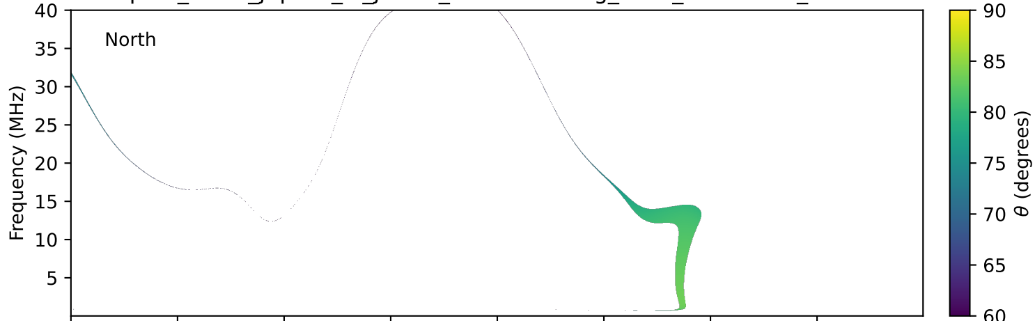
expres_earth_jupiter_io_jrm33_lossc-wid1deg_3kev_20250302_v11.cdf
