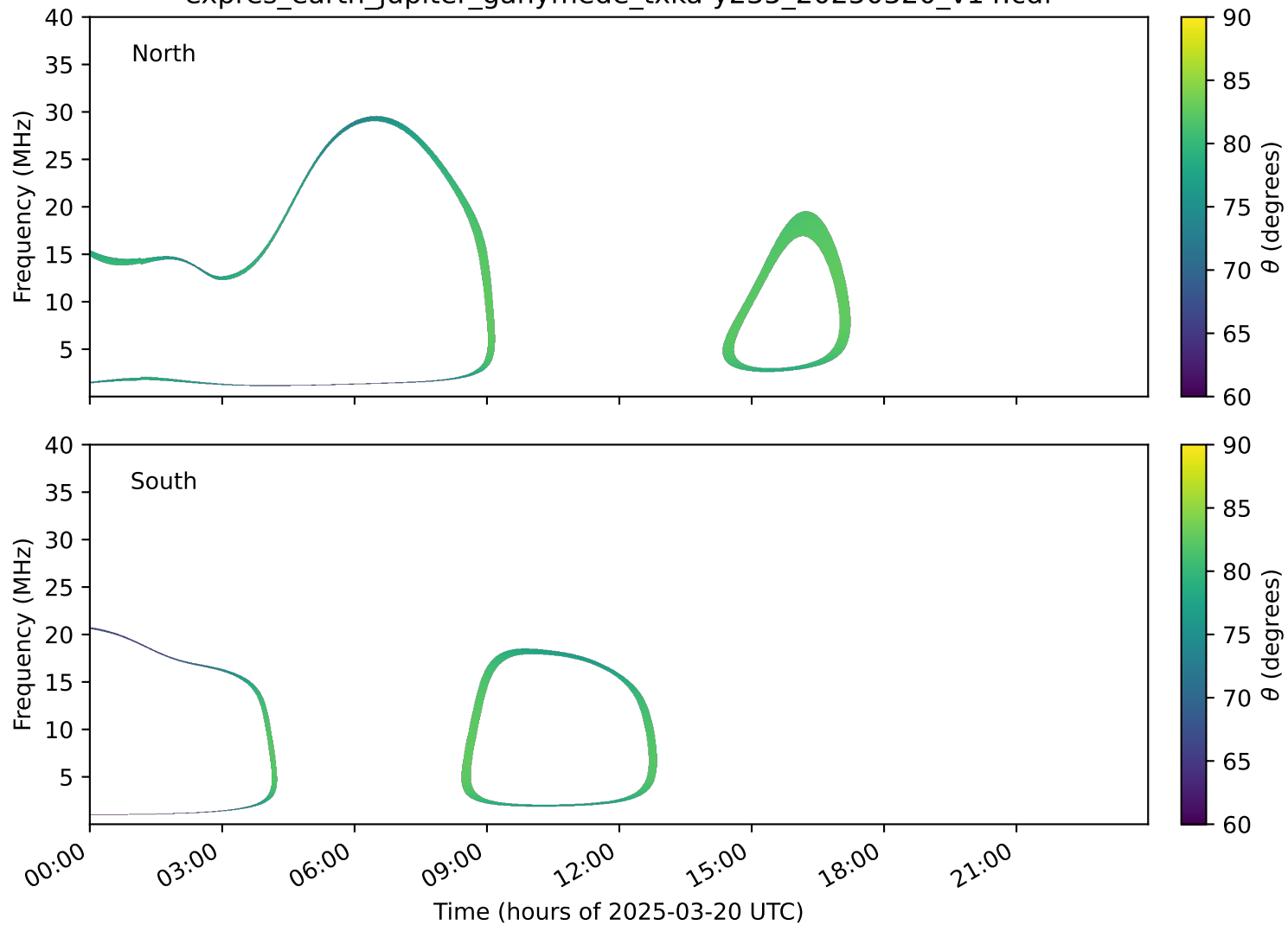
expres_earth_jupiter_ganymede_txka-y235_20250320_v14.cdf
